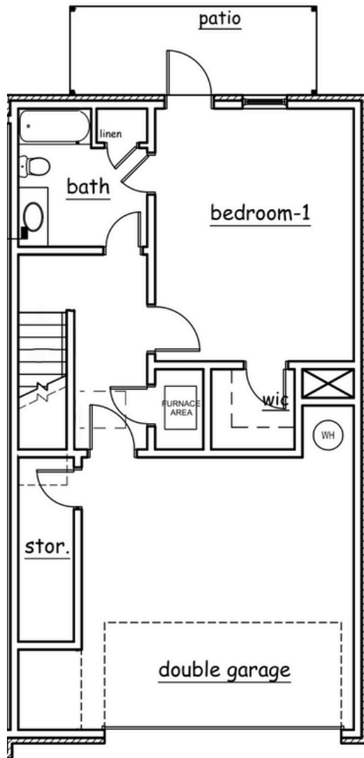
Lower Level Unit Plan
