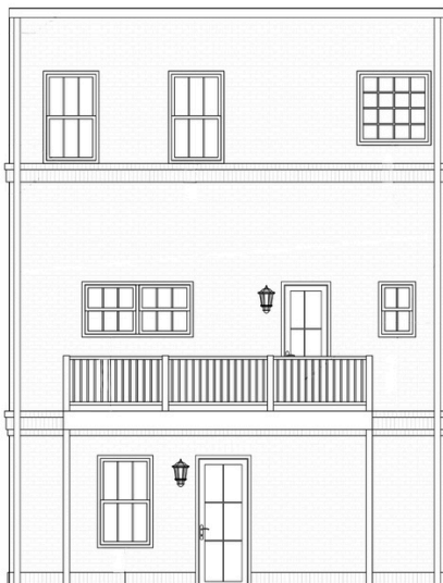
Enlarged Rear Ext Elev
